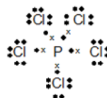
\text{PCl}_5
