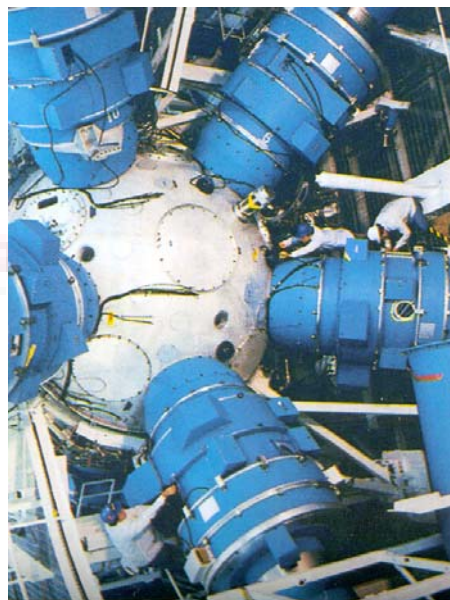
Stellarator
