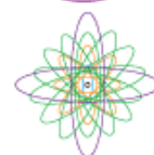
Orbitals
