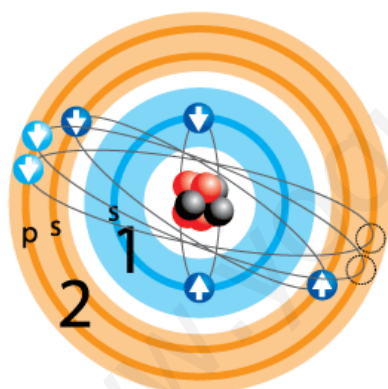
Carbono (C)
