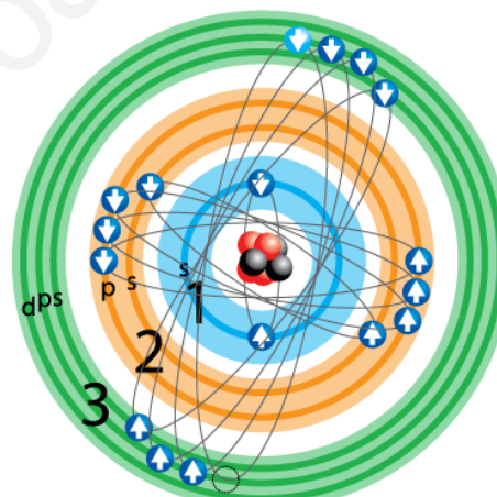
Cloro (Cl)
